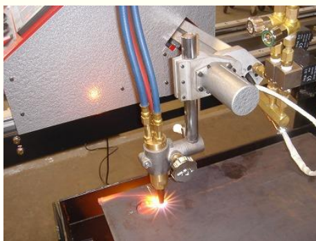
Single Oxy-fuel Torch
